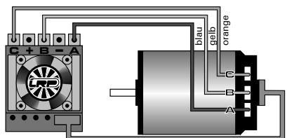
Hall-Sensor Kabel
