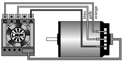
Hall-Sensor Kabel
