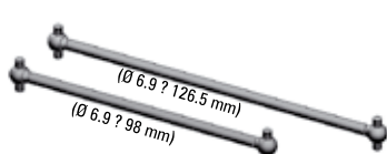
132236 Dogbone Middle Differential (f+r) - S8 TX RTR Antriebsknochen Mitteldifferential (v+h) - S8 TX RTR
